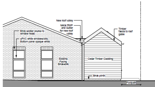
4 Proposed Side Elevation #1 1:50
