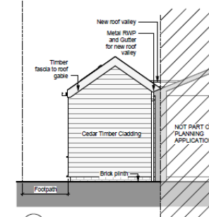
6 Proposed Side Elevation #2 1:50
